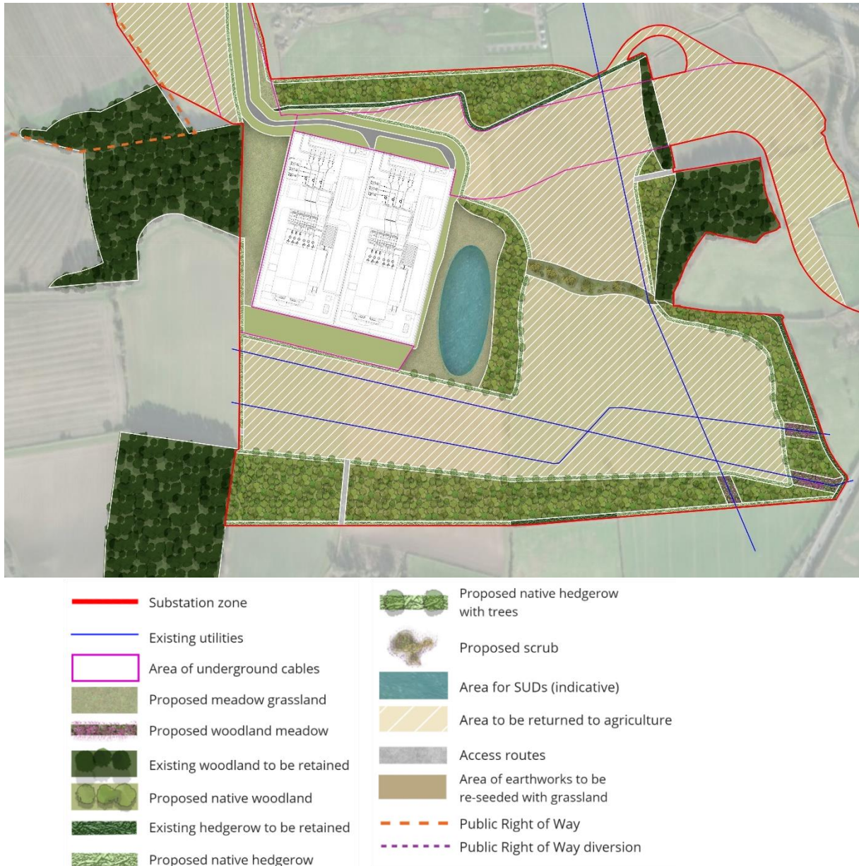
Plate 4-36 Indicative landscape mitigation plan
